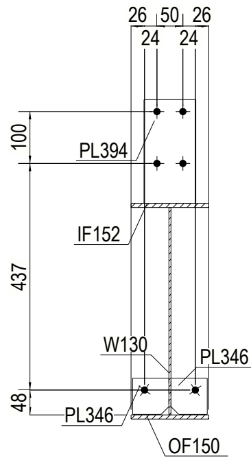
SEC A 1:10
