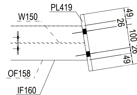
SEC B 1:10
